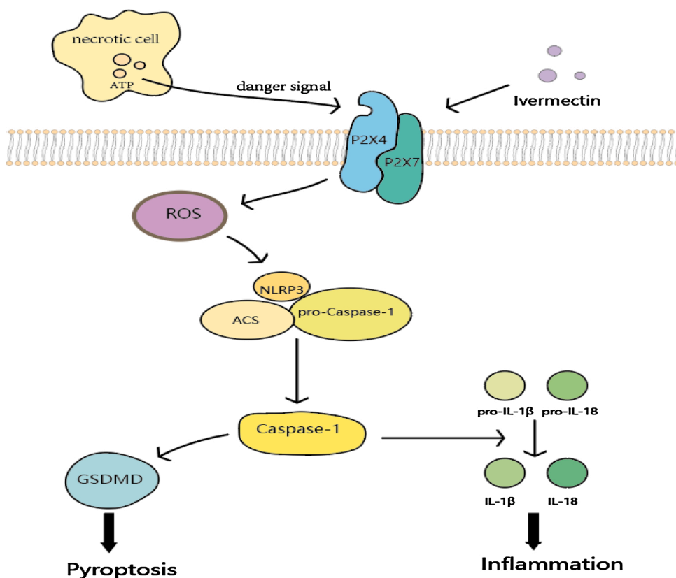
Fig. 4. Mechanisms of IVM-induced P2 \times 4/P2 \times 7 /NLRP3-mediated pyroptosis. IVM can promote ROS release in cancer cells by P2 \times 4/P2 \times 7 receptors. Cellular ROS can activate NLRP3 Inflammasome including ASC, NLRP3 and pro-caspase-1 assemble. Subsequently, NLRP3 Inflammasome initiates pro-caspase-1 to self-shear into mature caspase-1. On the one hand, activated caspase-1 induces the secretion of pro-inflammatory cytokines IL-1 \beta and IL-18. On the other hand, caspase-1 activated by GSDMD triggers pyroptosis independent of apoptosis.
